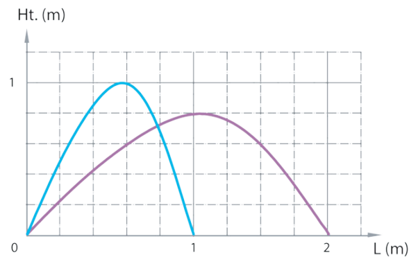
Water Parabolas
